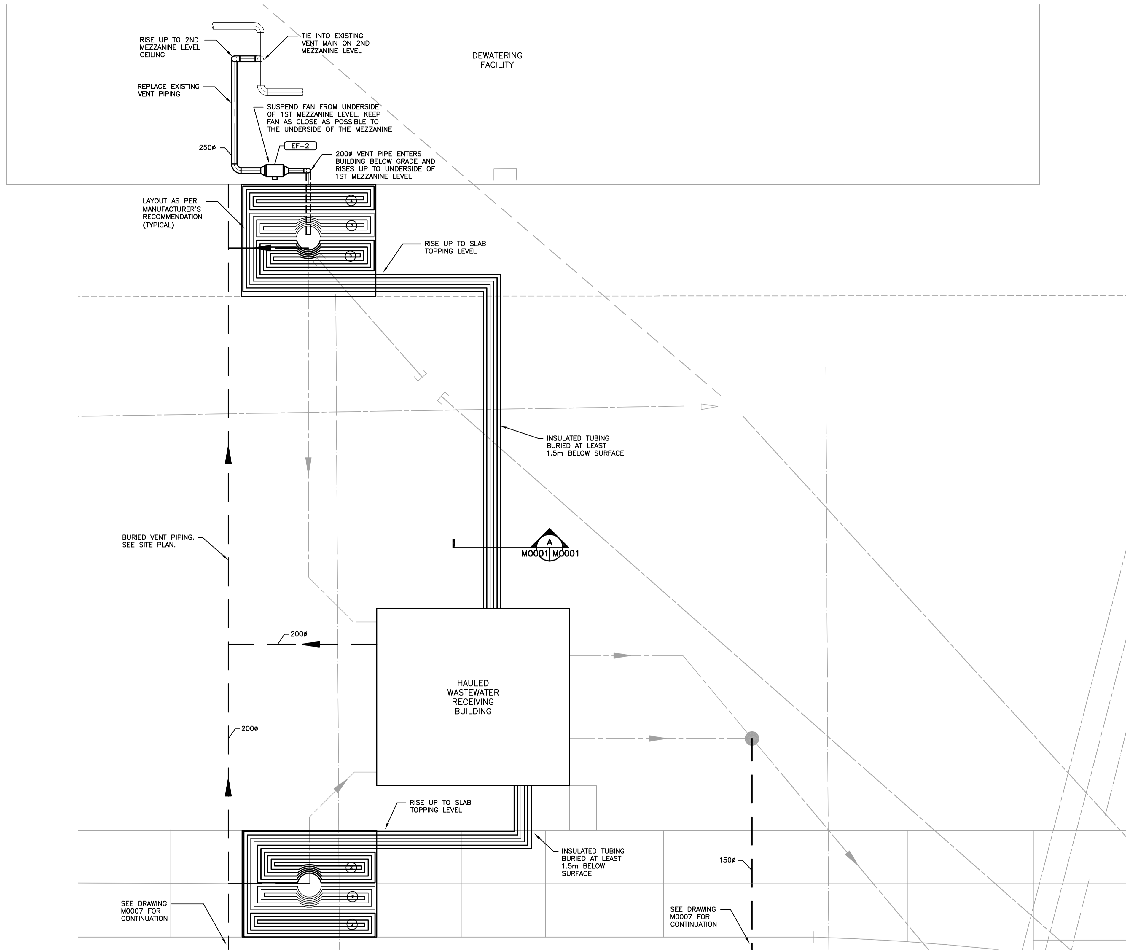
1 MECHANICAL SITE PLAN M0001 1:100
