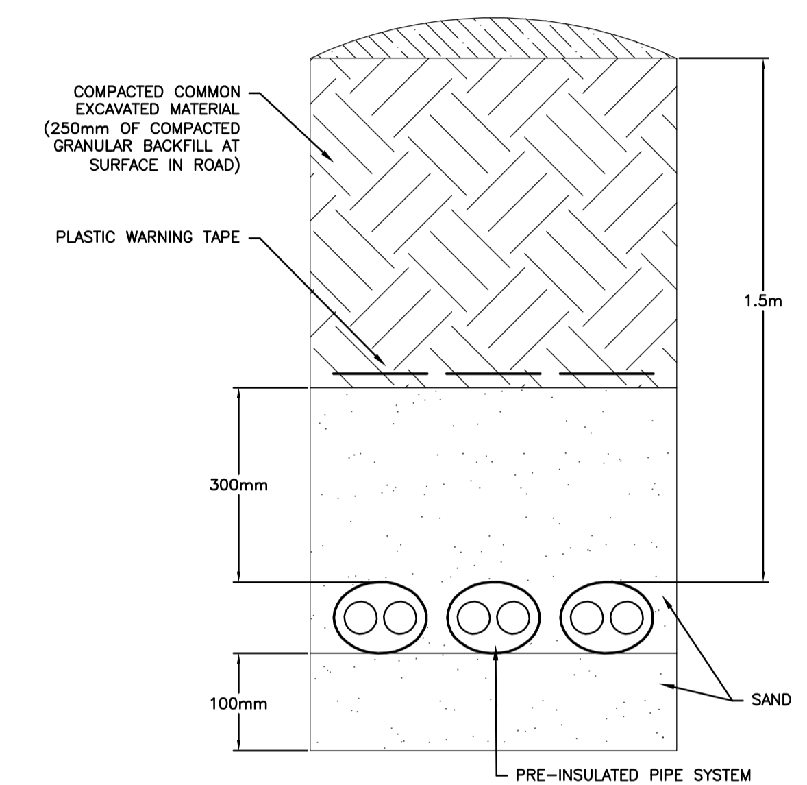
A BURIED HYDRONIC PIPING M0001 NTS
